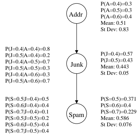
Fig. 4. A Bayesian network modeling dependencies in utilities for giving away address, receiving junk mail, and receiving spam
